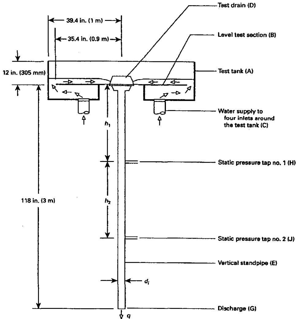
Fig. 1 Resistance Value Apparatus
