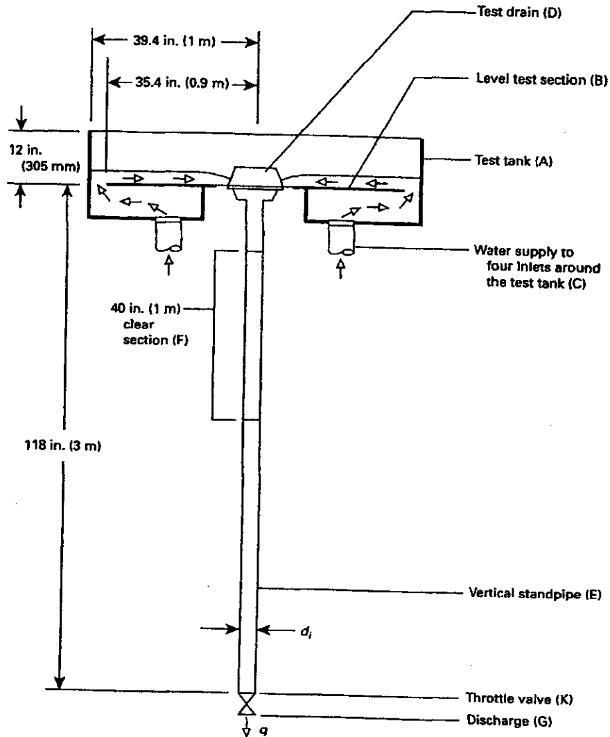
Fig. 2 Depth Versus Flow Apparatus
