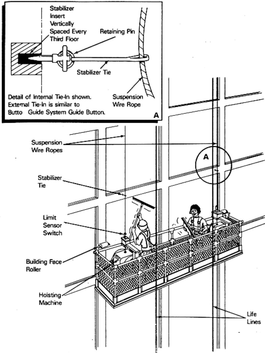
Figure 2. Typical Self-Powered Platform – Intermittent Tie-In System
