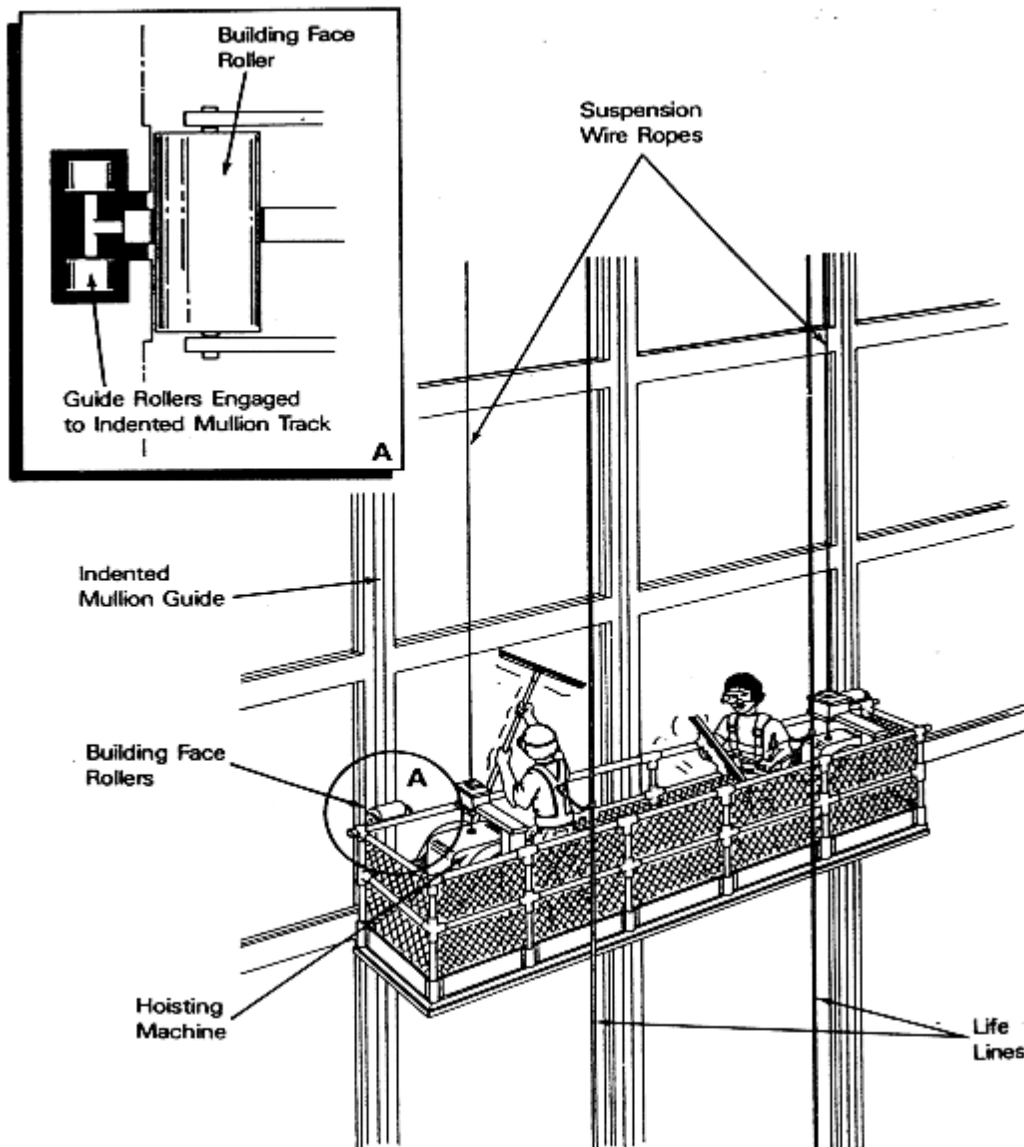
Figure 1. Typical Self-Powered Platform – Continuous External or Indented Mullion Guide System
